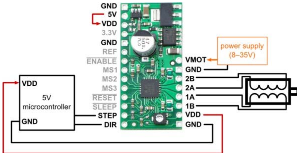
Minimal wiring diagram for wiring a 5V microcontroller to an A4983/A4988 stepper motor driver carrier with voltage regulators (full-step mode).
